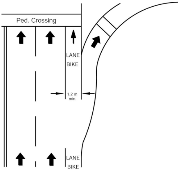
(1) RIGHT-TURN-ONLY LANE
